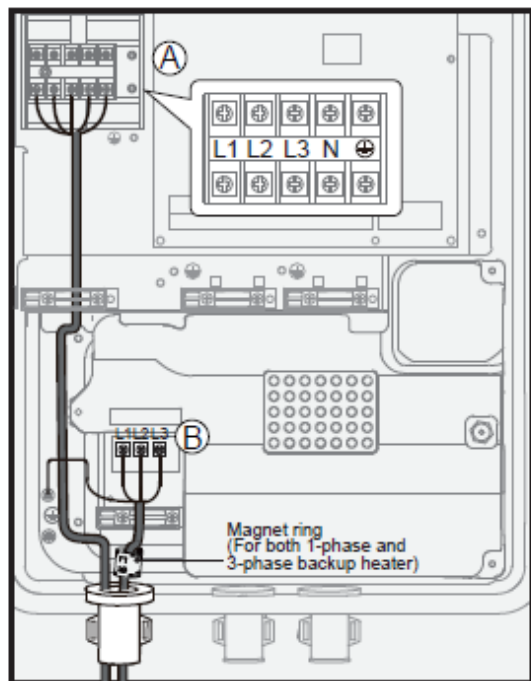
12, 16 kW model
