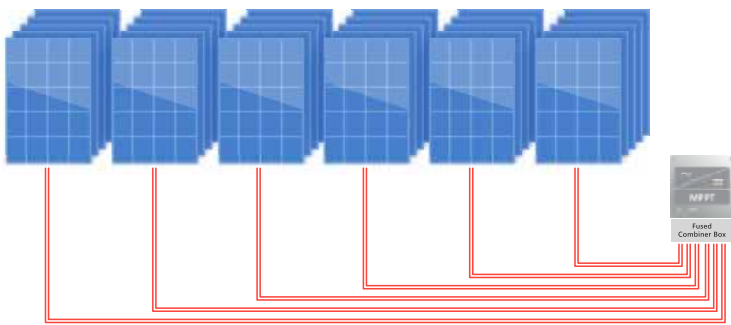
■ Traditional inverter
